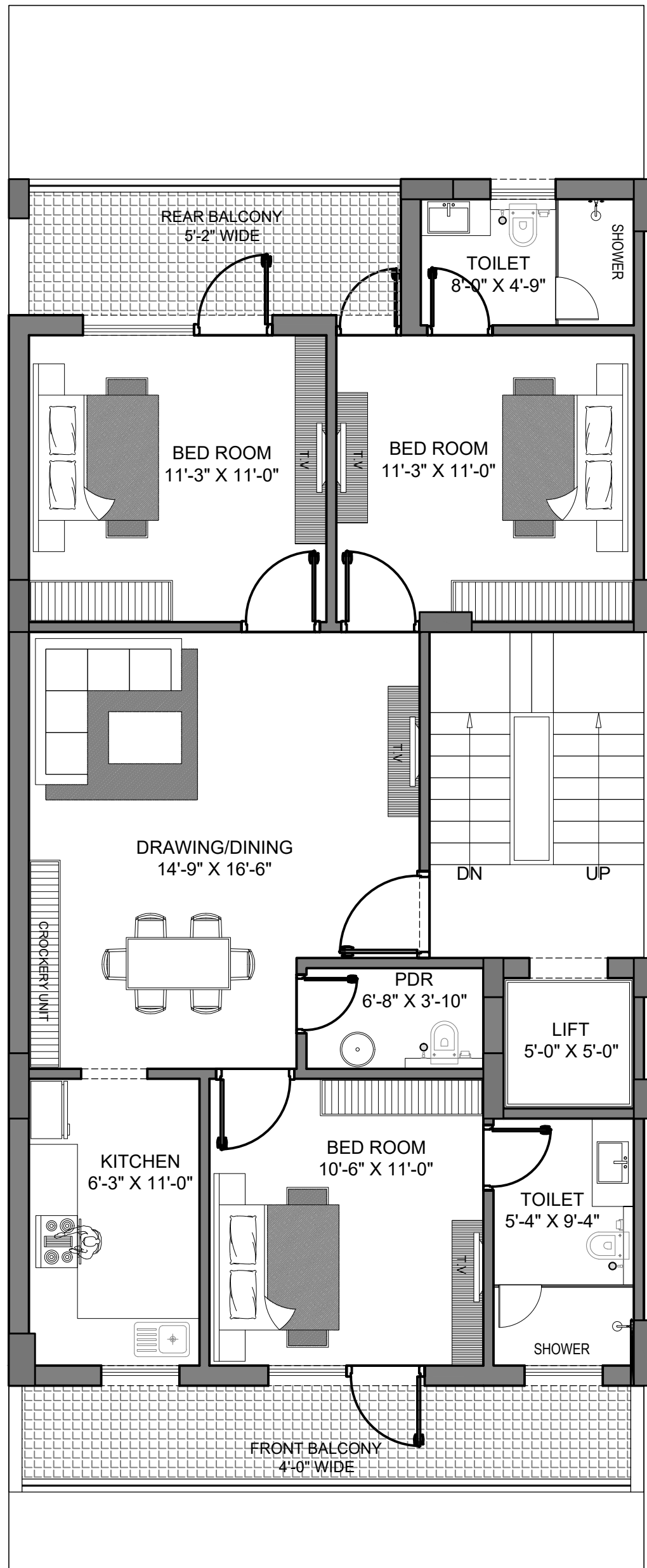
TYPICAL FLOOR PLAN TYPE-A
